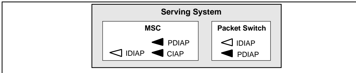
Figure 13: Mobile Intercept Subject's Serving System IAPs
