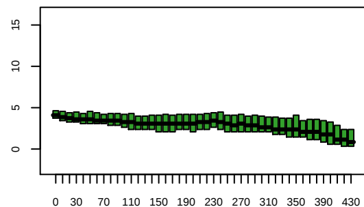
\log(\text{green intensity})
