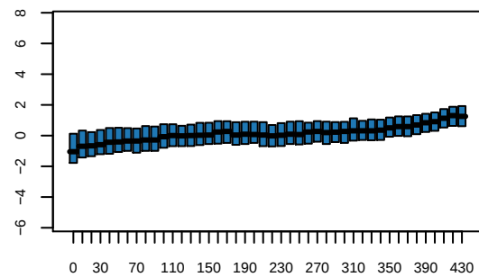
\log(\text{ratio})
